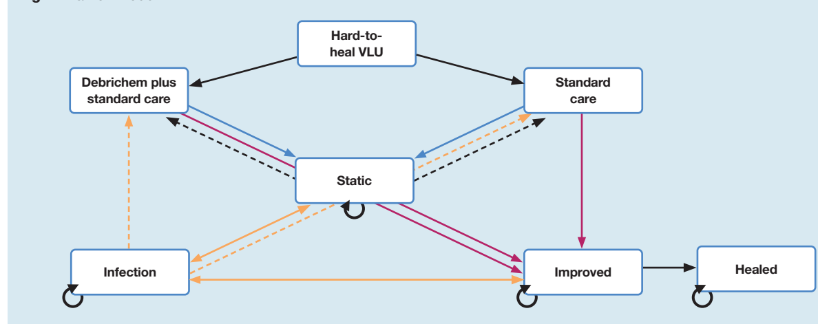
Fig 1. Markov model
